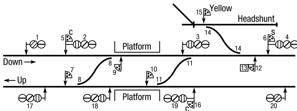
FIGURE 2-2 Typical Through Station with Colour Light Signalling.
