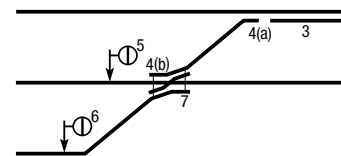
FIGURE 2-5 Double Slip Variation.
